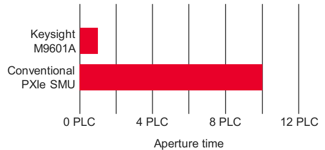
Figure 3. Aperture time required to achieve 30 fArms current measurement noise
