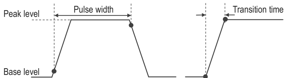
Figure 7. Definition of the pulse parameters and the transition time
