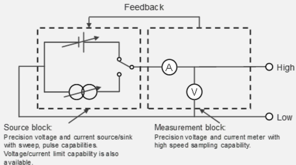
Figure 1. Simplified block diagram of the M9601A
