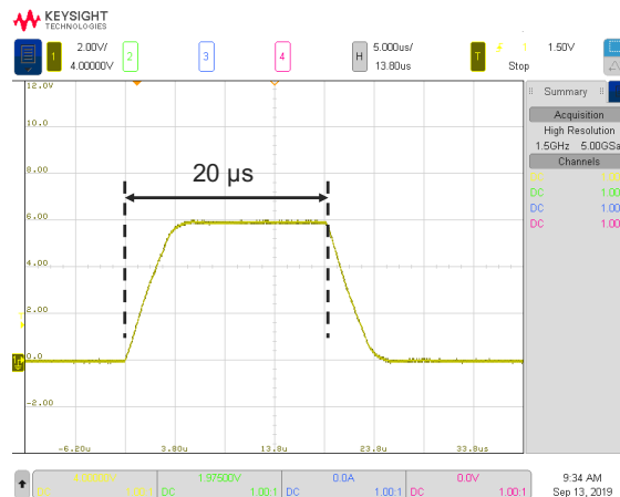
Figure 4. Narrow pulse down to 20 \mu s enables you to suppress self-heat effect to reveal the true characteristics of the devices
